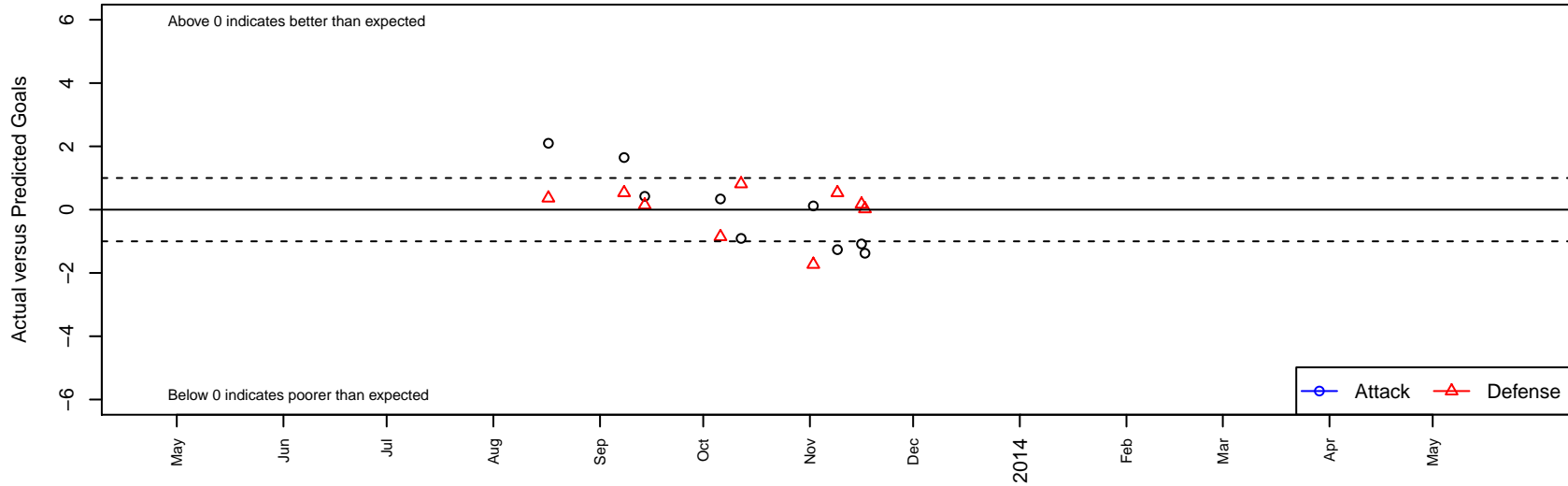
Merced United FC G00 Dots are actual minus expected GF (blue circles) and GA (red triangles). Blue line is smoothed change in attack strength. Red is smoothed change in defense strength.
